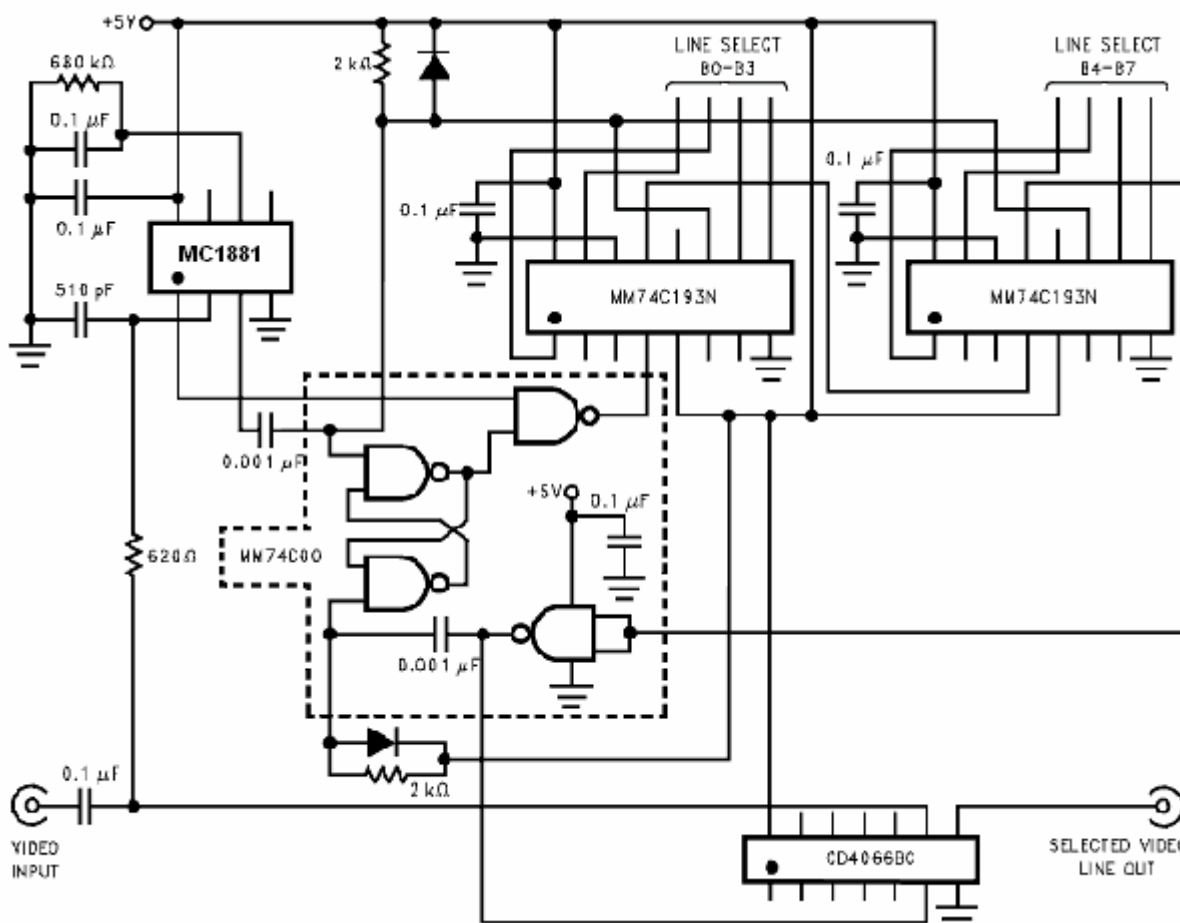
FIGURE 3. Video Line Selector MC1881, MC1881-X
