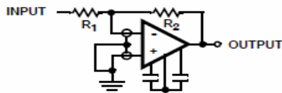
FIGURE 1A. INVERTING AMPLIFIER
