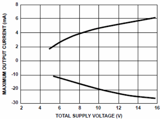
FIGURE 9. MAXIMUM OUTPUT CURRENT vs SUPPLY VOLTAGE
