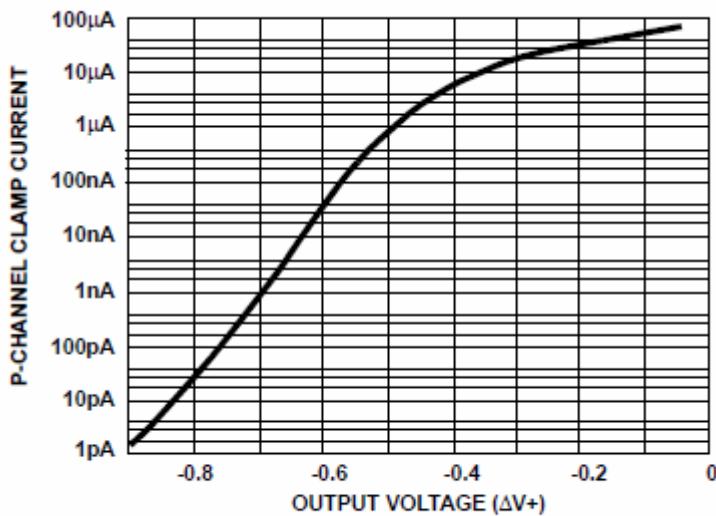
FIGURE 21. P-CHANNEL CLAMP CURRENT vs OUTPUT VOLTAGE
