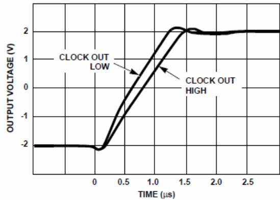
FIGURE 18. VOLTAGE FOLLOWER LARGE SIGNAL PULSE RESPONSE (NOTE)
