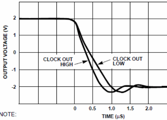
FIGURE 19. VOLTAGE FOLLOWER LARGE SIGNAL PULSE RESPONSE (NOTE)
