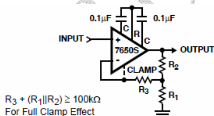
FIGURE 2. NON INVERTING AMPLIFIER WITH OPTIONAL CLAMP
