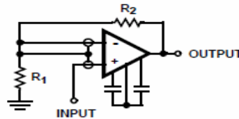
FIGURE 1C. NON-INVERTING AMPLIFIER FIGURE 1. CONNECTION OF INPUT GUARDS
