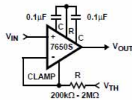
FIGURE 5. LOW OFFSET COMPARATOR
