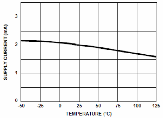
FIGURE 8. SUPPLY CURRENT vs AMBIENT TEMPERATURE
