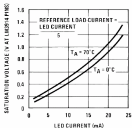
LED Driver Saturation Voltage
