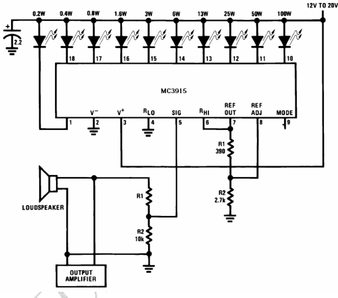
Audio Power Meter
