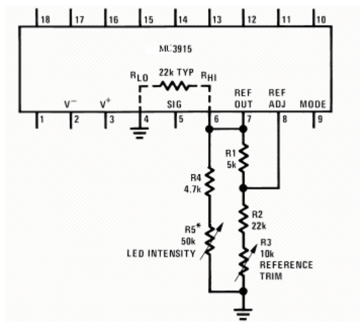
FIGURE 8. Varying LED Intensity
