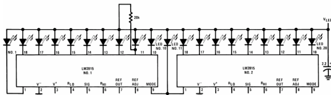
Cascading LM3915s in Dot Mode
