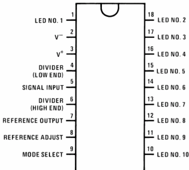
Dual-in-Line Package
