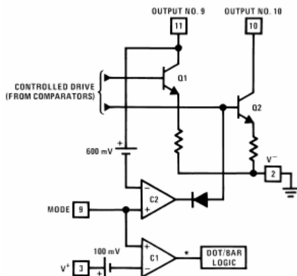
Block Diagram of Mode Pin Function
