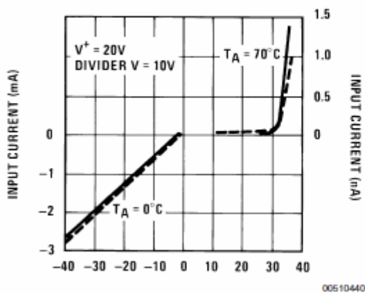
Input Current Beyond Signal Range (Pin 5)
