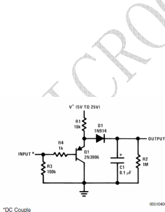
FIGURE 1. Half-Wave Peak Detector
