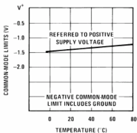
Common-Mode Limits
