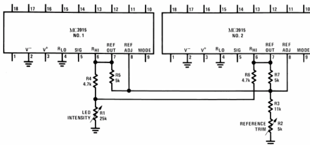
FIGURE 9. Independent Adjustment of Reference Voltage and LED Intensity for Multiple MC3915s
