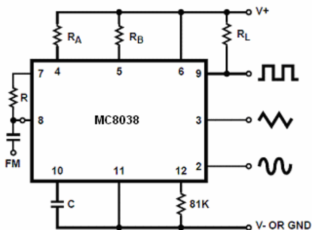
FIGURE 5A. CONNECTIONS FOR FREQUENCY MODULATION
