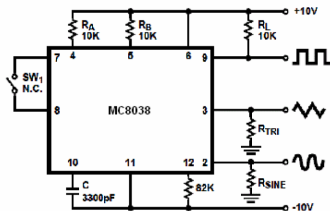
FIGURE 1. TEST CIRCUIT
