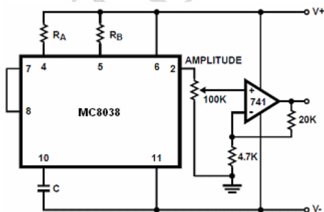
FIGURE 6. SINE WAVE OUTPUT BUFFER AMPLIFIERS
