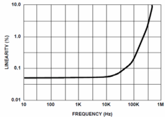
FIGURE 18. TRIANGLE WAVE LINEARITY vs FREQUENCY
