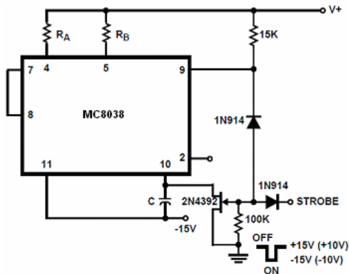
FIGURE 7. STROBE TONE BURST GENERATOR
