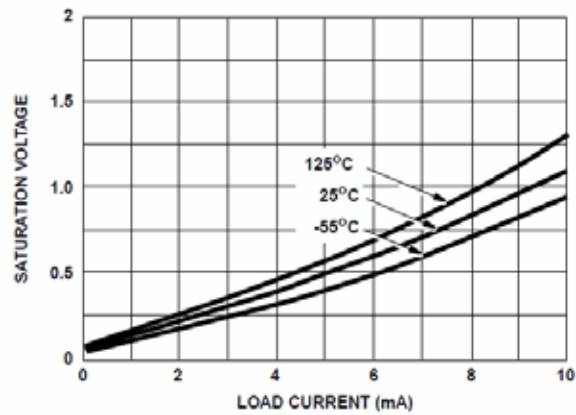
FIGURE 15. SQUARE WAVE SATURATION VOLTAGE vs LOAD CURRENT
