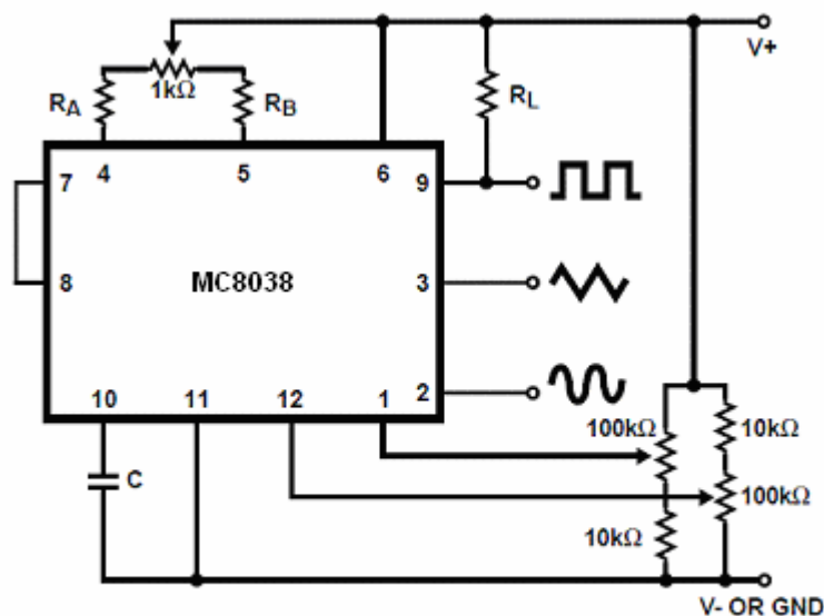
FIGURE 4. CONNECTION TO ACHIEVE MINIMUM SINE WAVE DISTORTION
