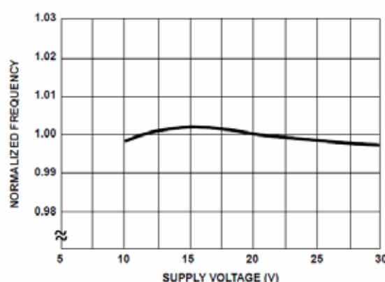
FIGURE 12. FREQUENCY vs SUPPLY VOLTAGE
