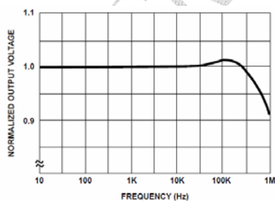
FIGURE 19. SINE WAVE OUTPUT VOLTAGE vs FREQUENCY
